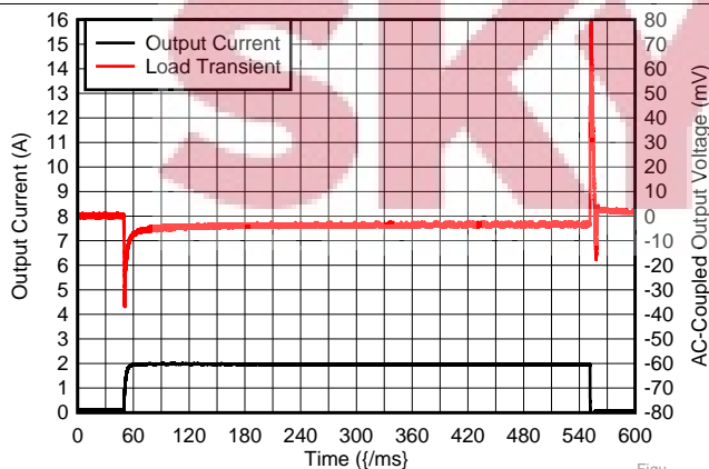
Figure 29. Load Transient Response ( V_{OUT} = 1.2\text{ V} )
